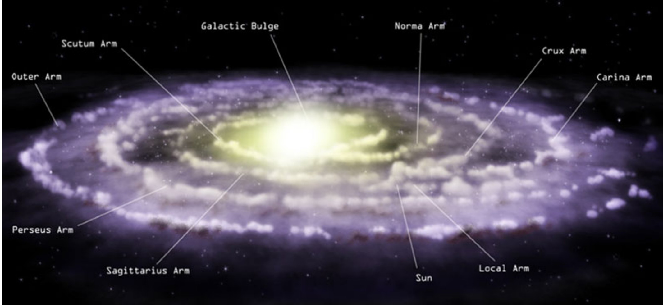
An Artist's illustration of the Milky Way Galaxy
