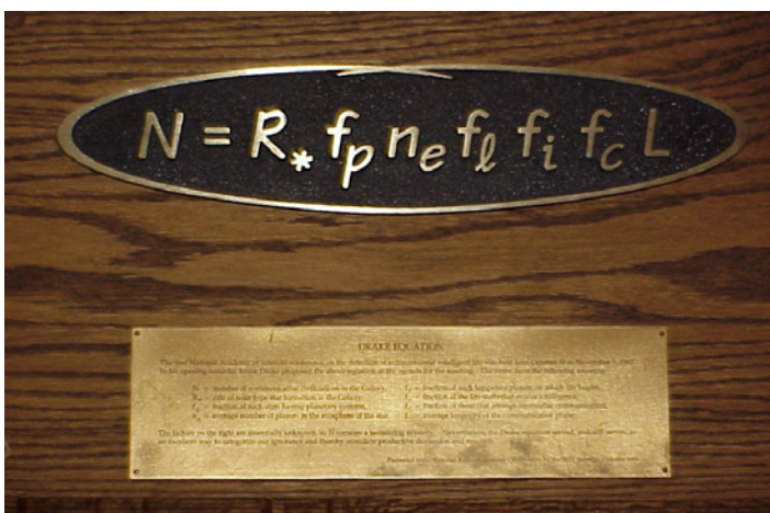
Drake equation plaque in the NRAO Green Bank Residence Hall Lounge. Note the smudges from so many people touching the plaque. Credit: NRAO/NSF/AUI.
